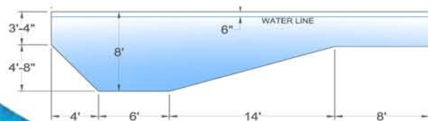
Hopper bottom, variable water depth with deep end
